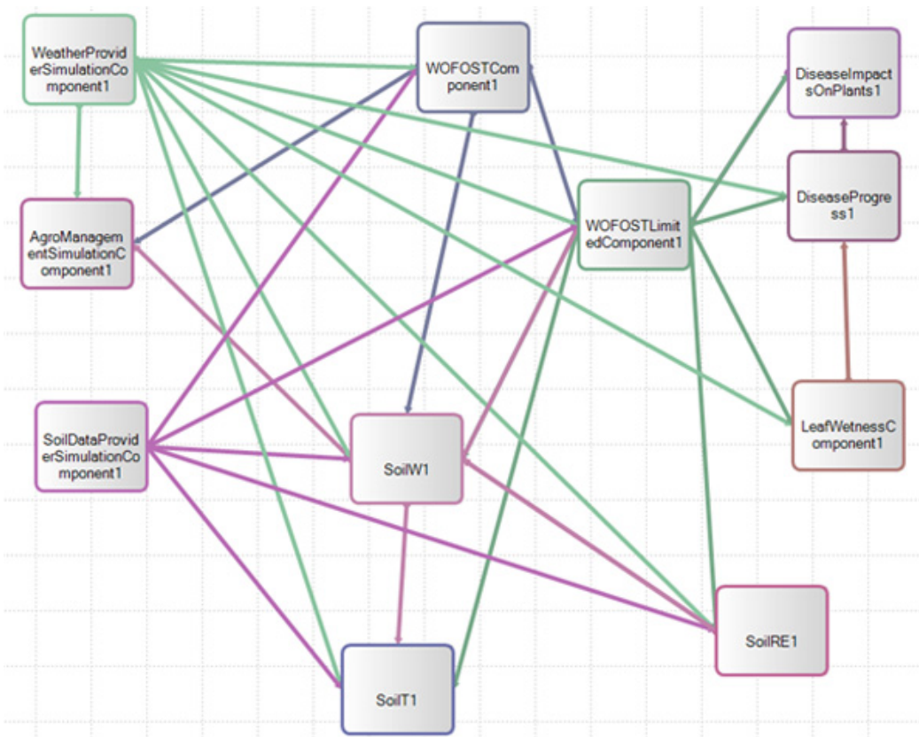
Figure 2 Wofost - Connections between all components (including optional components)
